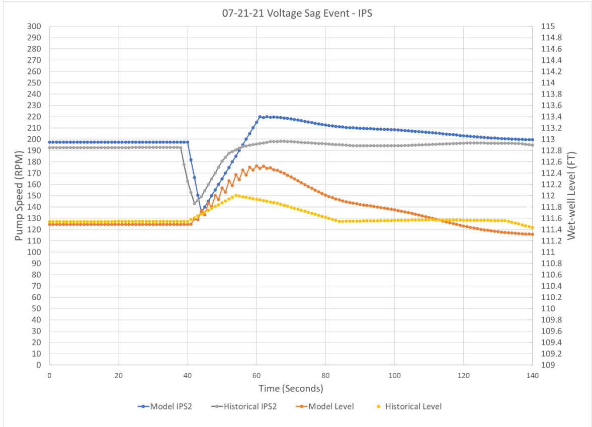
Figure 3. Model versus historical data for Voltage Sag on July 21, 2021. One IPS pump was online and pumping approximately 65 mgd prior to the voltage sag.
